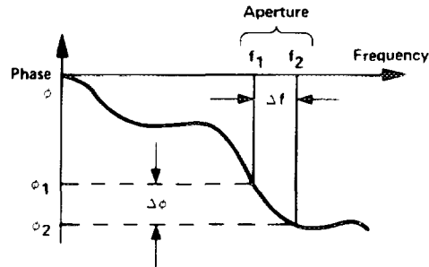
Figure 4-7. Rate of Phase Change Versus Frequency
