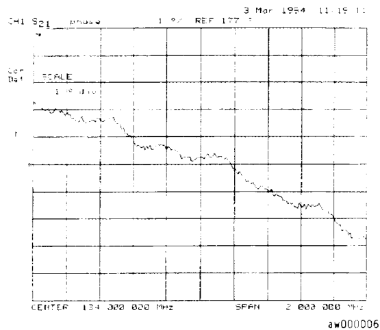
Figure 4-12. Deviation From Linear Phase Example Measurement
