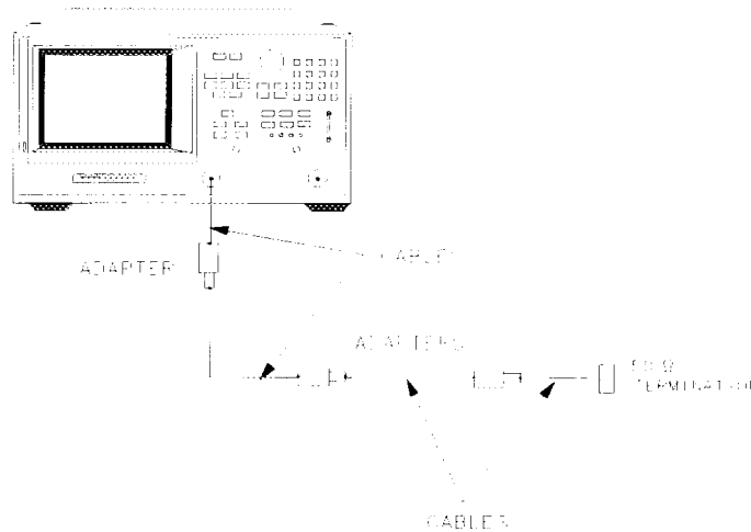
Figure 4-21. Device Connections for Reflection Time Domain Measurement
