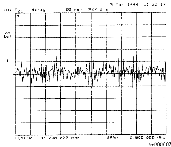
Figure 4-13. Group Delay Example Measurement
