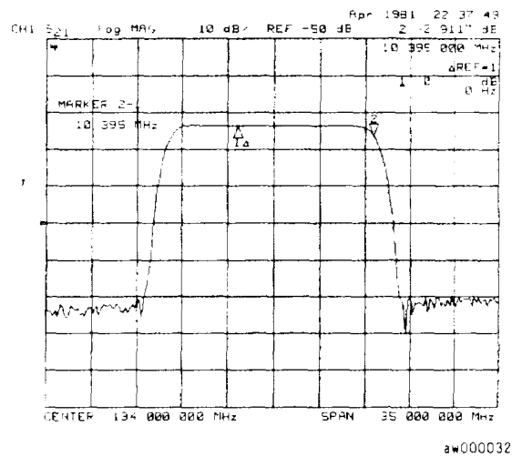
Figure 7-9. Example of Marker 1 as the Reference Marker
