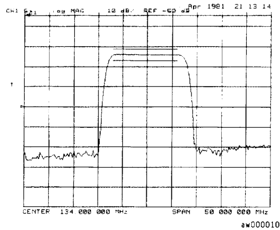
Figure 10-2. Example Flat Limit Line
