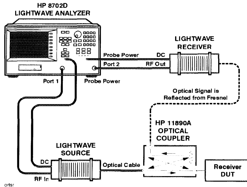
Figure 3-2. Optical Reflection Test Setup
