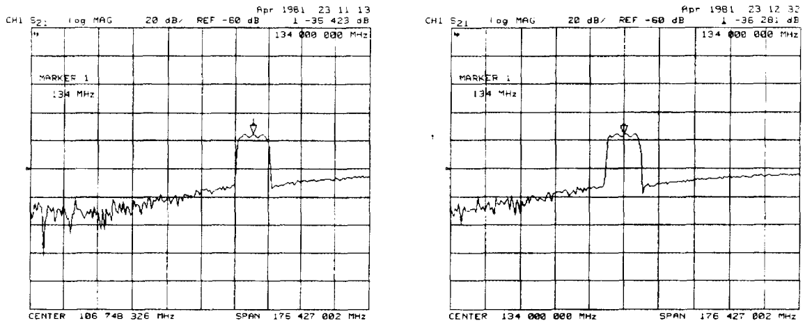
Figure 7-5. Example of Setting the Center Frequency Using a Marker
