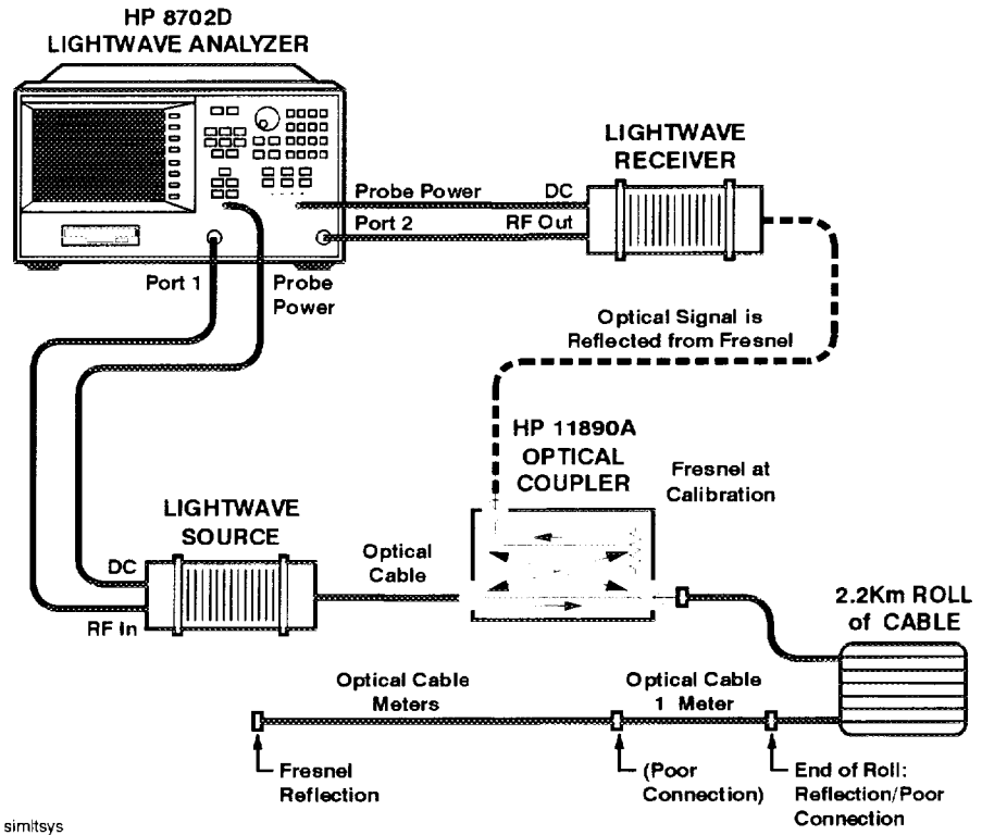
simitsys Figure 5-5. Simulated Lightwave System Fault Location Configuration
