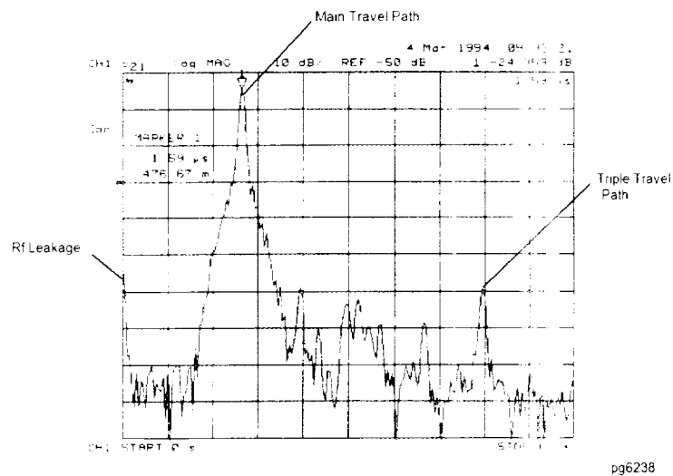
Figure 4-16. Time Domain Transmission Example Measurement
