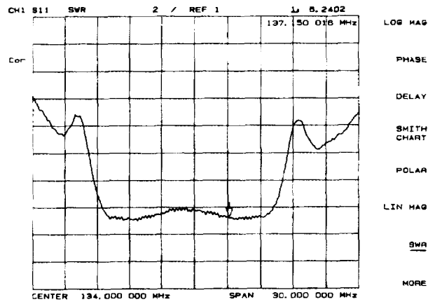
Figure 7-18. Example Standing-Wave-Ratio Measurement Trace
