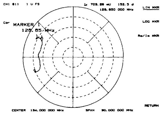
Figure 6-6. Polar Format
