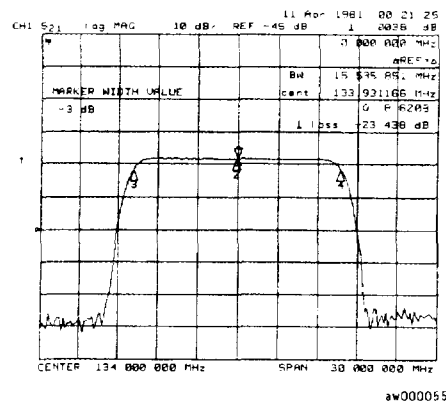
Figure 7-15. Example Measurement of 3 dB Bandwidth
