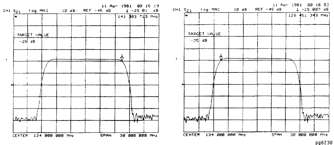
Figure 7-10. Example of Searching for a Target Amplitude Using a Marker
