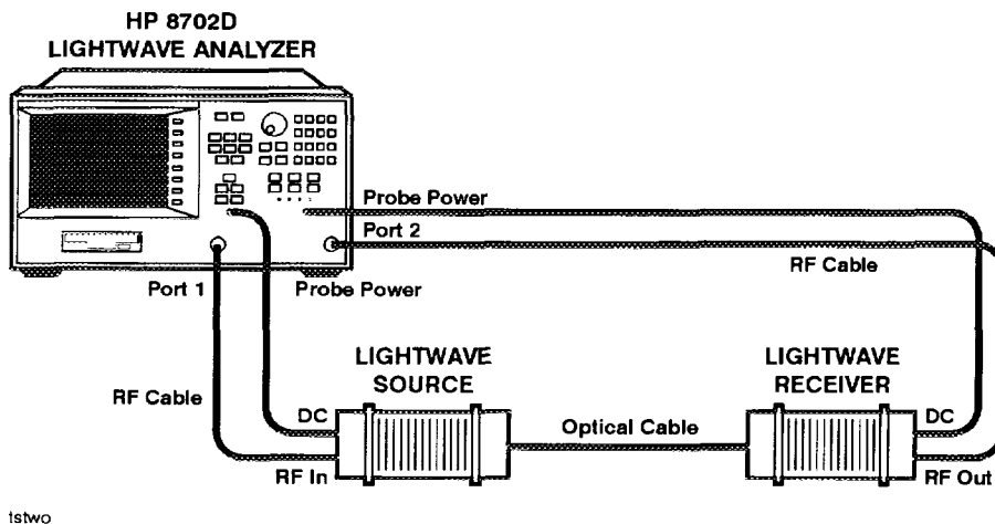
Figure 1-7. Calibration with lightwave receiver
