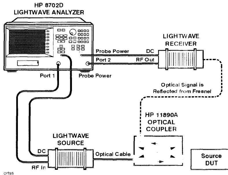
Figure 2-3. Optical Reflection Test Setup
