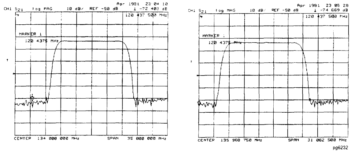
Figure 7-3. Example of Setting the Start Frequency Using a Marker
