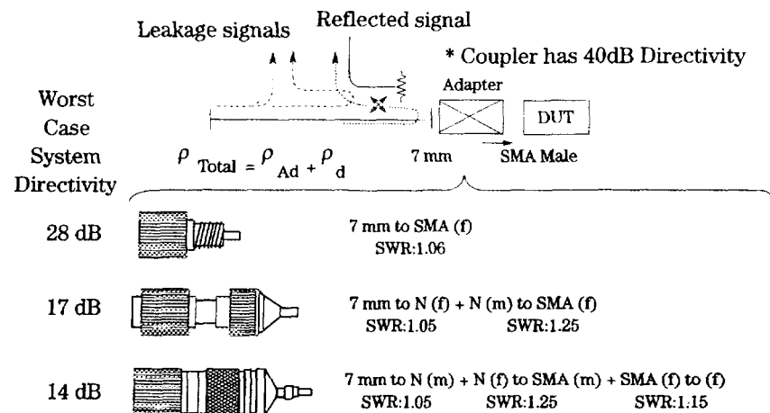
Figure 4-47. Adapter Considerations
