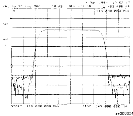
Figure 4-17. Gating Effects in a Frequency Domain Example Measurement
