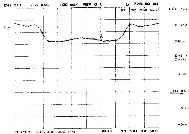
Figure 7-17. Example Reflection Coefficient Measurement Trace
