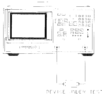
Figure 6-18. Typical Harmonic Mode Test Setup
