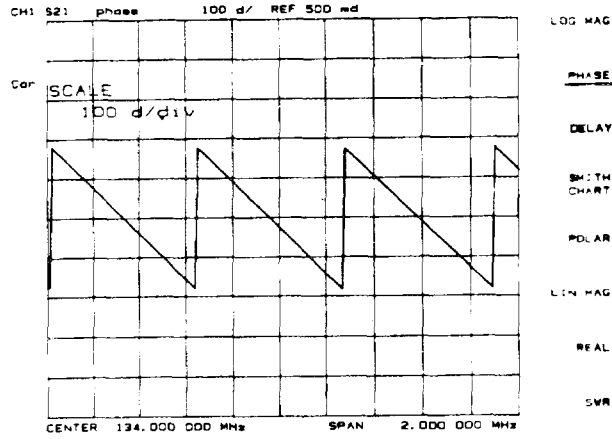
Figure 6-3. Phase Format
